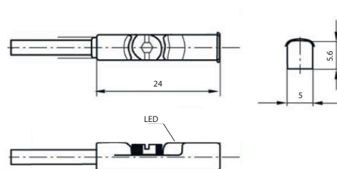
Dimensions [mm]
